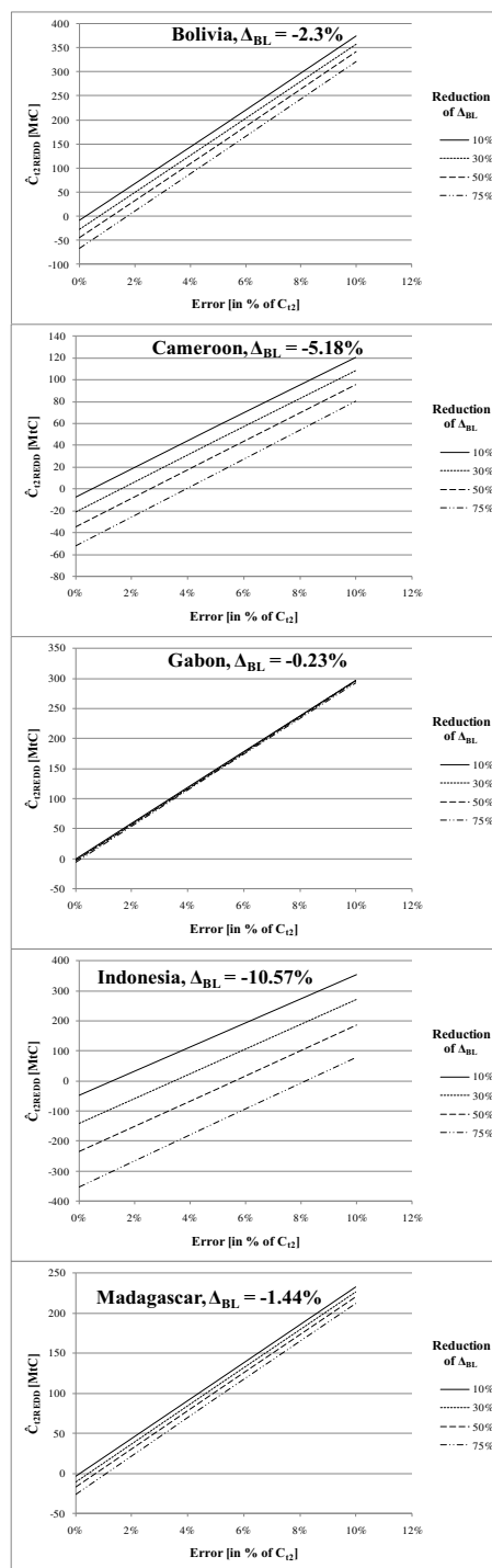
Figure 1 Graphs of resulting \hat{C}_{t2REDD} (in tC \cdot 10^6 ) for five selected countries in relation to error at time 2, ( E_{t2} ) for different reduction scenarios for \Delta_{BL} showing the effect of total error and deforestation and degradation rates on carbon credits; positive numbers display emissions, negative numbers removals.
