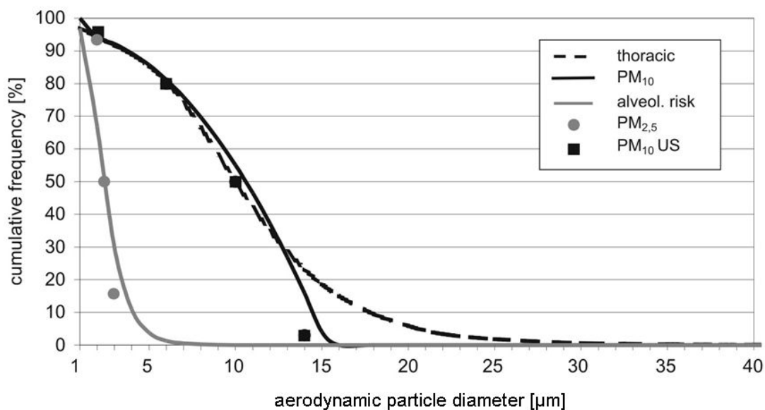
Figure A1–1 Sampling criteria for inhalable, thoracic and respirable particles expressed as percentage of TSP
