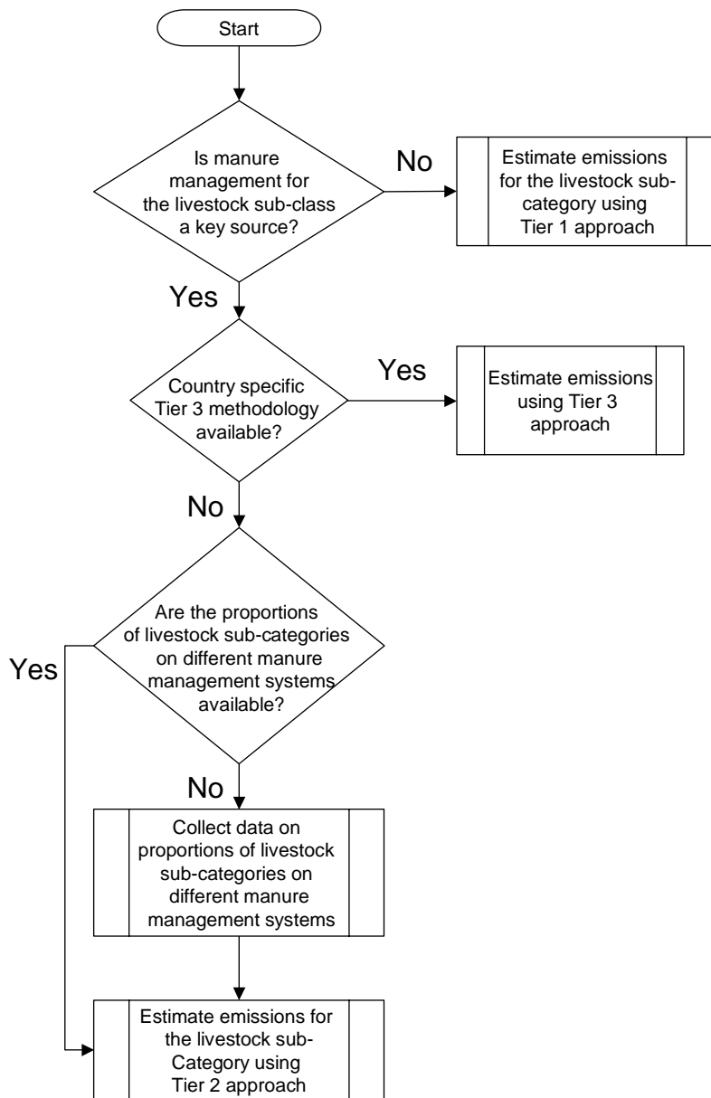
Figure 3-1 Decision tree for source category 4.B Animal husbandry and manure management
