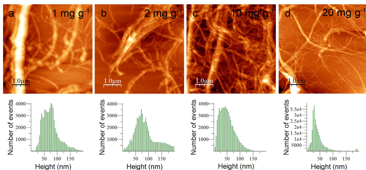
Figure 3. AFM imaging of LPMO-treated cellulose. (Top) AFM topography images, and (bottom) height distribution of cellulose fibers treated with LPMO at different enzyme concentrations ( 1\text{--}20\text{ mg g}^{-1} ) after dispersion.
