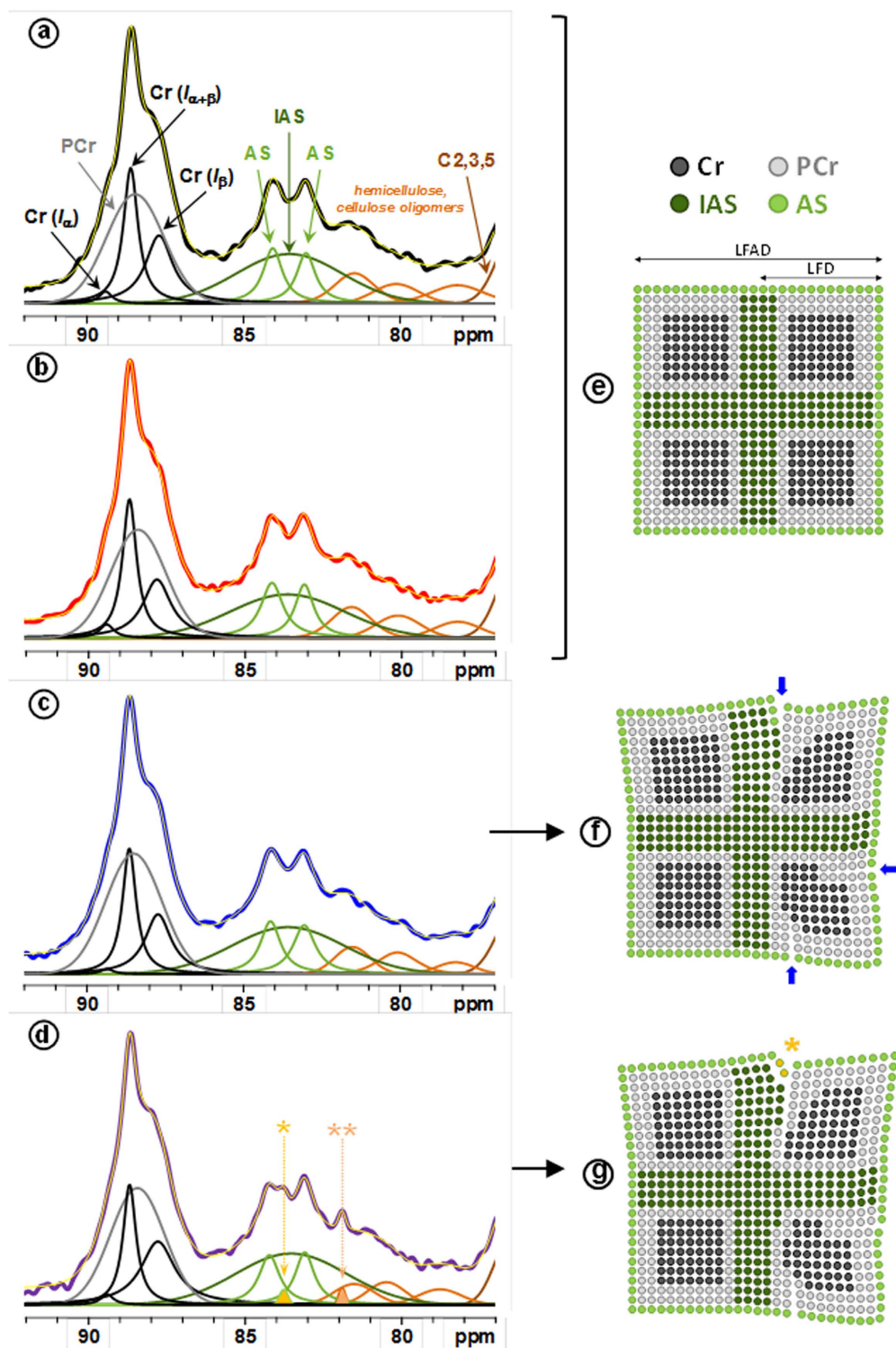
Figure 5. Solid-state ^{13}\text{C} CP/MAS NMR spectra. Left: Deconvolution of C-4 region with crystalline forms \text{Cr}(I_{\alpha}) , \text{Cr}(I_{\beta}) and \text{Cr}(I_{\alpha+\beta}) (black), para-crystalline form (PCr) (grey), accessible fibril surfaces (AS) (green), and inaccessible fibril surface (IAS) (dark green) signals for reference cellulose fibers (a) before and (b) after dispersion, and for cellulose fibers submitted to the LPMO treatment (c) before and (d) after dispersion. Four signals from hemicelluloses and/or cellulose oligomers are indicated in orange. Yellow line in (a,b,c and d) corresponds to the sum of individual peaks resulting from the spectral deconvolution. In spectrum (d), two additional peaks are denoted by (*) and (**) (see text for details). Right: Schematic representation of cellulose fibril model for (e) reference cellulose fibers, and LPMO-treated cellulose fibers (f) before and (g) after dispersion. The number of points in the scheme is proportional of the area of the corresponding NMR signals. Blue arrows represent possible nicking points created by the LPMO on the cellulose. Fibril scheme displays the different cellulose forms: lateral fibril dimension (LFD), and lateral fibril aggregate dimensions (LFAD).
