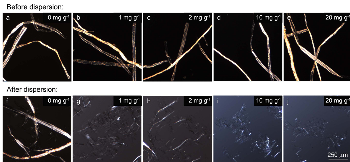
Figure 2. Morphology of LPMO-treated cellulose. Optical microscopy images of cellulose fibers after LPMO treatment at different enzyme concentrations ( 1\text{--}20\text{ mg g}^{-1} ) (b–e) before and (g–j) after dispersion. Images of reference samples (without LPMO treatment) have been included for non-dispersed and dispersed fibers (a and f, respectively).
