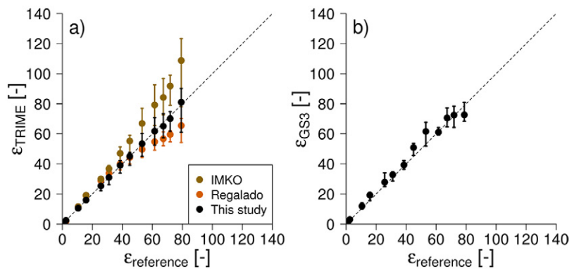
Fig. 2. Median and the 2.5 to 97.5% quantiles of all measured dielectric permittivities ( \epsilon ) with (a) TRIME ( \epsilon_{\text{TRIME}} ) or (b) GS3 ( \epsilon_{\text{GS3}} ) probes vs. the reference dielectric permittivity ( \epsilon_{\text{reference}} ). Dashed line is the 1:1 line.
