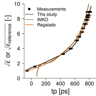
Fig. 1. Square root of the (i) reference dielectric permittivity \sqrt{\epsilon_{\text{reference}}} vs. measured “pseudo transit times” ( t_p ) and (ii) relationship of t_p and square root of the dielectric permittivity ( \sqrt{\epsilon} ) derived from Eq. [2], [3], and [4].
