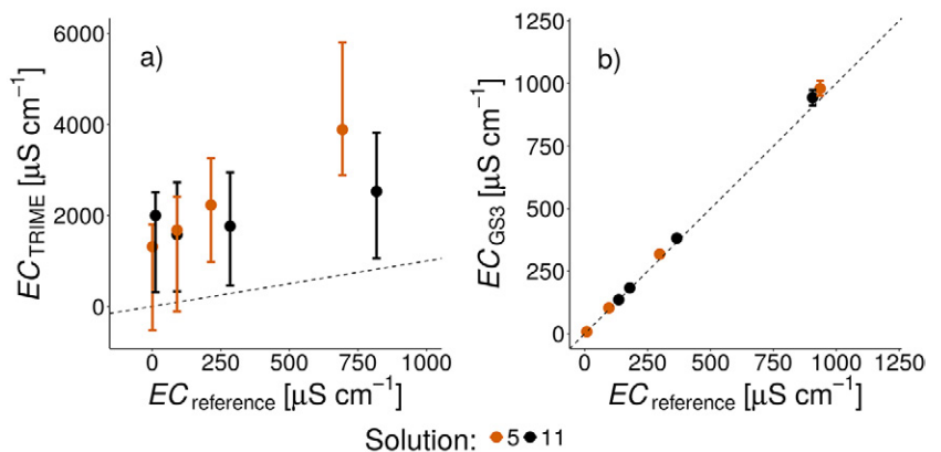
Fig. 4. Median and the 2.5 to 97.5% quantiles of all measured electrical conductivities with (a) the TRIME probes ( \text{EC}_{\text{TRIME}} ) and (b) the GS3 probes ( \text{EC}_{\text{GS3}} ) vs. the reference electrical conductivities ( \text{EC}_{\text{reference}} ). Dashed line is the 1:1 line.
