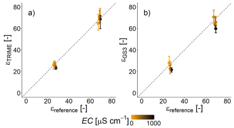
Fig. 3. Median and the 95% variability of measured dielectric permittivities ( \epsilon ) with (a) TRIME ( \epsilon_{\text{TRIME}} ) or (b) GS3 ( \epsilon_{\text{GS3}} ) probes vs. the reference dielectric permittivity ( \epsilon_{\text{reference}} ) under different electrical conductivities (EC) ( \mu\text{S cm}^{-1} ) with Solutions 5 and 11. Dashed line is the 1:1 line.
