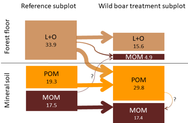
Figure 5. Changes in different soil organic carbon (SOC) pools in the forest floor (L and O horizons) and the underlying mineral soil (0–10 cm depth) due to bioturbation. Average carbon stocks for all 23 plots (Mg SOC ha -1 ). POM: particulate organic matter, MOM: mineral-associated organic matter.
