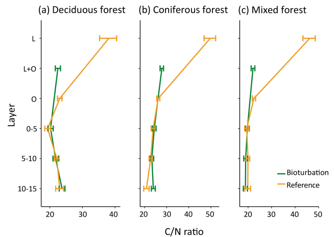
Figure 6. Mean carbon : nitrogen (C/N) ratio of organic matter in different forest floor layers and mineral soil layers in disturbed and reference plots in deciduous ( n = 6 ), coniferous ( n = 11 ) and mixed forest ( n = 6 ). Bars indicate standard error.
