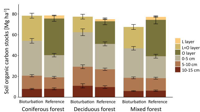
Figure 3. Mean soil organic carbon (SOC) stock ( \text{Mg ha}^{-1} ) in different layers and depth increments with treatment mimicking wild boar grubbing (Bioturbation) with undisturbed control (Reference) for three different forest types. Differences in total SOC stocks were not significantly different between the forest types.
