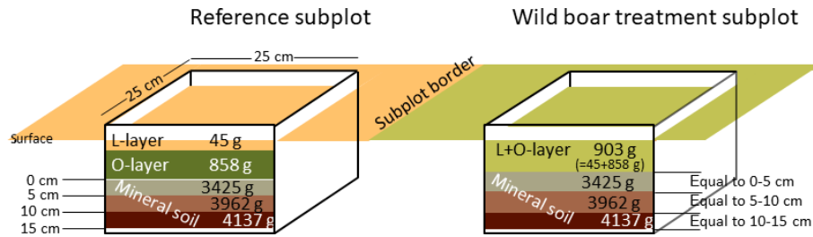
Figure 1. Equal mass sampling of forest floor (L and O layer) and mineral soil (0–15 cm depth). Weights refer to the mean weight of the different layers and soil depth increments as obtained in the field.
