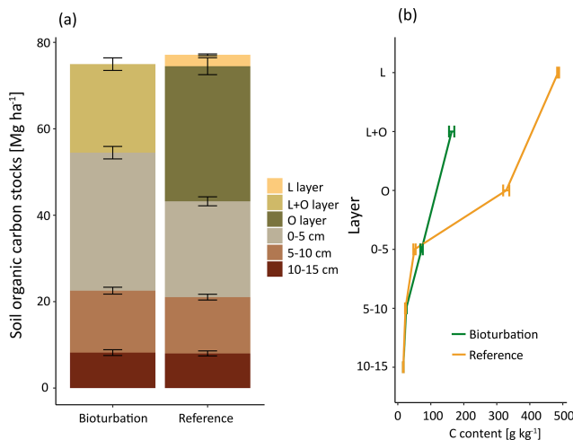
Figure 2. (a) Mean soil organic carbon (SOC) stock ( \text{Mg ha}^{-1} ) distribution, significant differences were found in 0–5 cm depth and in the combined forest floor (L + O layer). (b) SOC content ( \text{g kg}^{-1} ) in different layers and soil depth increments for plots in the treatment mimicking wild boar grubbing (Bioturbation) and in the undisturbed control subplots (Reference).
