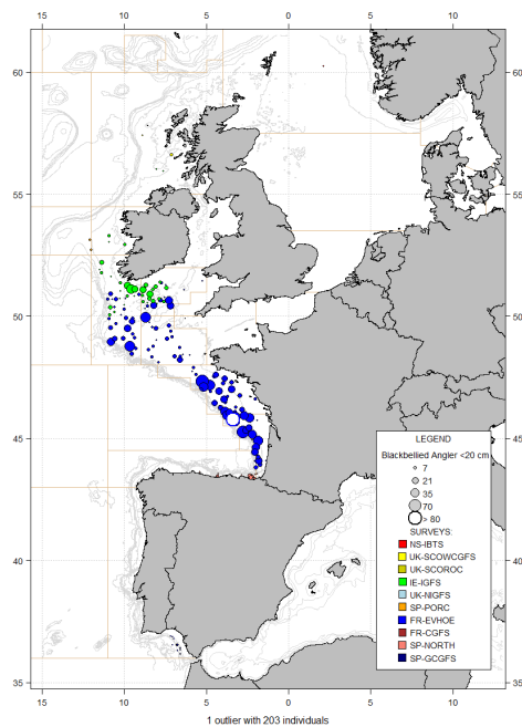
Figure A.6.20. Catches in numbers per hour of 0-group black-bellied anglerfish, Lophius americanus (<20 cm), in summer/autumn 2020 IBTSurveys.
