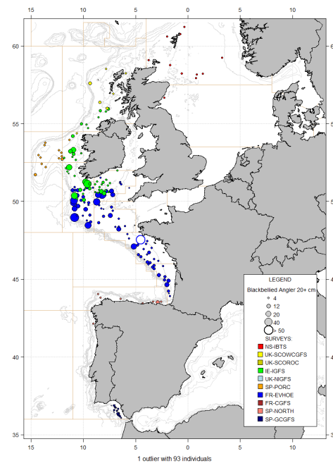
Figure A.6.21. Catches in numbers per hour of 1+ group black-bellied anglerfish, Lophius americanus (≥20 cm), in summer/autumn 2020 IBTSurveys.
