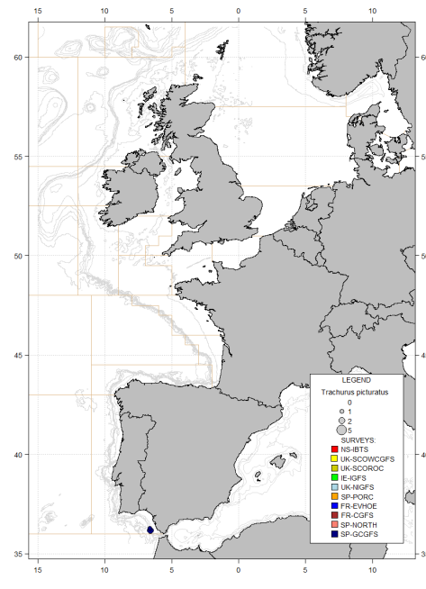
Figure A.6.43. Catches in numbers per hour per hour of blue jack mackerel, Trachurus picturatus , in summer/autumn 2020 IBTSurveys.
