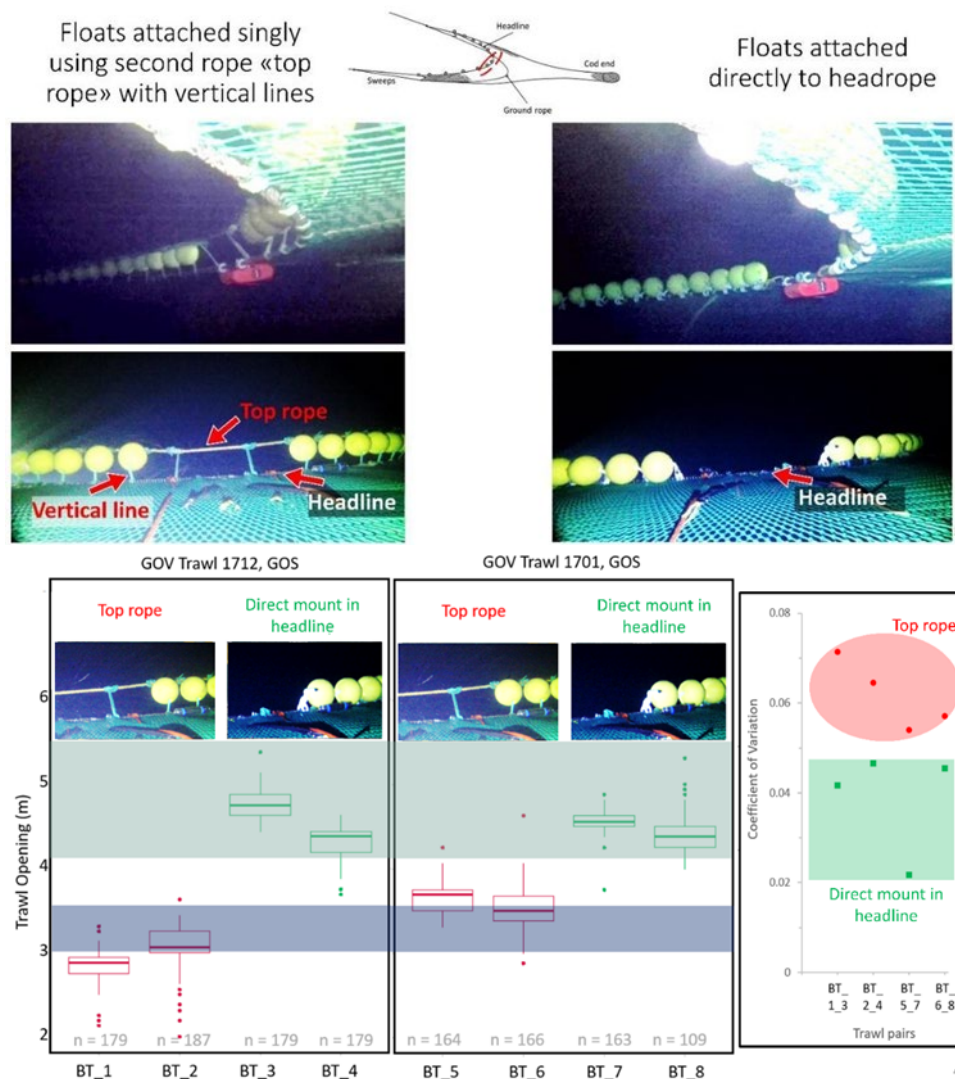
Figure 4.2.1. Underwater images and trawl opening results from GOV trials attaching the floats directly to the headrope or not.
