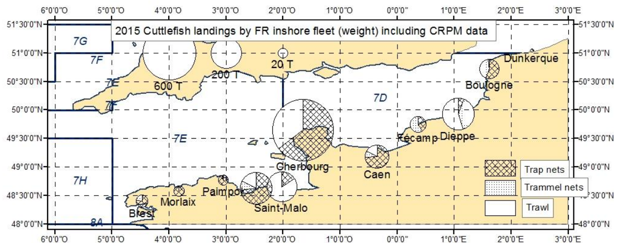
Figure 6: English Channel inshore fishery landings by France from the 3 main fishing gears (trawl, trap and trammel net), by fishing harbour (2015 official fishery statistics supplemented by "Comité des Pêches").
