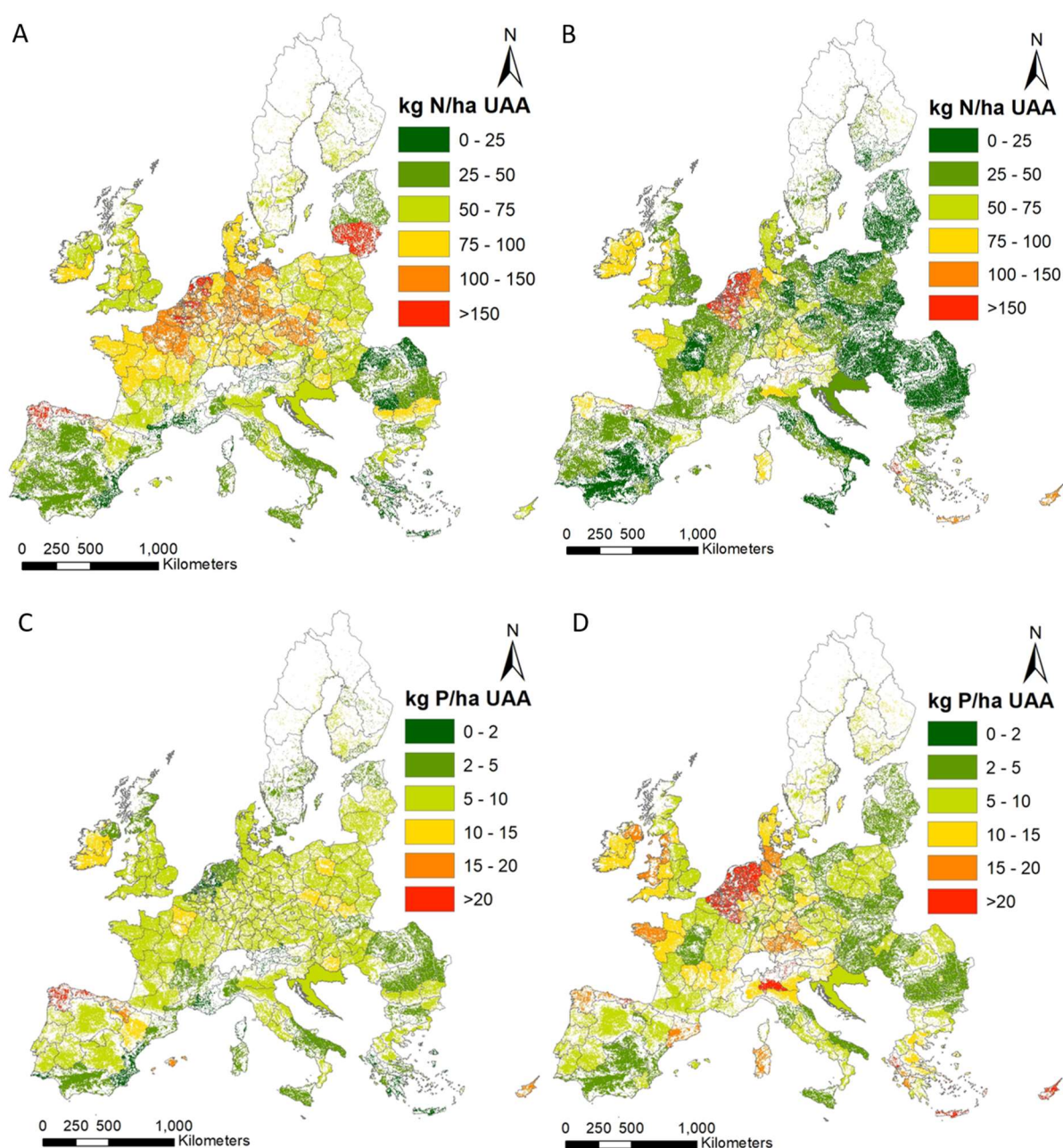
Figure 3.6 Application of nitrogen as synthetic fertilizer (A) and as manure (B), and the application of phosphorus (P) as synthetic fertilizer (C) and as manure (D). (Source MITERRA-Europe data)
