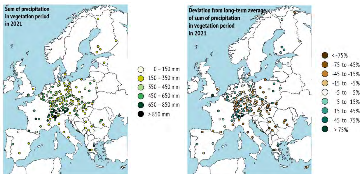
Figure 6-10: Precipitation (in mm (l/m²)) in the vegetation period in 2021 and deviation (in %) of the precipitation in the vegetation period in 2021 from the long-term average (1990–2020) on Level II plots.
