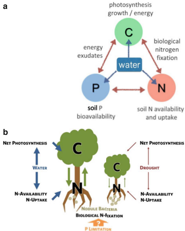
Fig. 32.3 (a) Water is the most critical factor for the interactions among carbon (C), nitrogen (N), and phosphate in soil-plant systems. (b) Schematic illustration of the interactions and transport of N and C with good water supply and drought stress (modified after Gypser and Veste 2019)
